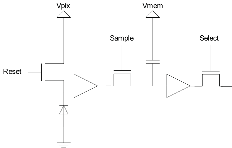
Figure 4. 6T-Pixel Architecture.
