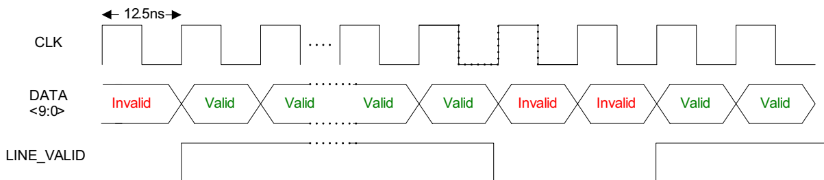
Figure 19. LINE_VALID Timing.
