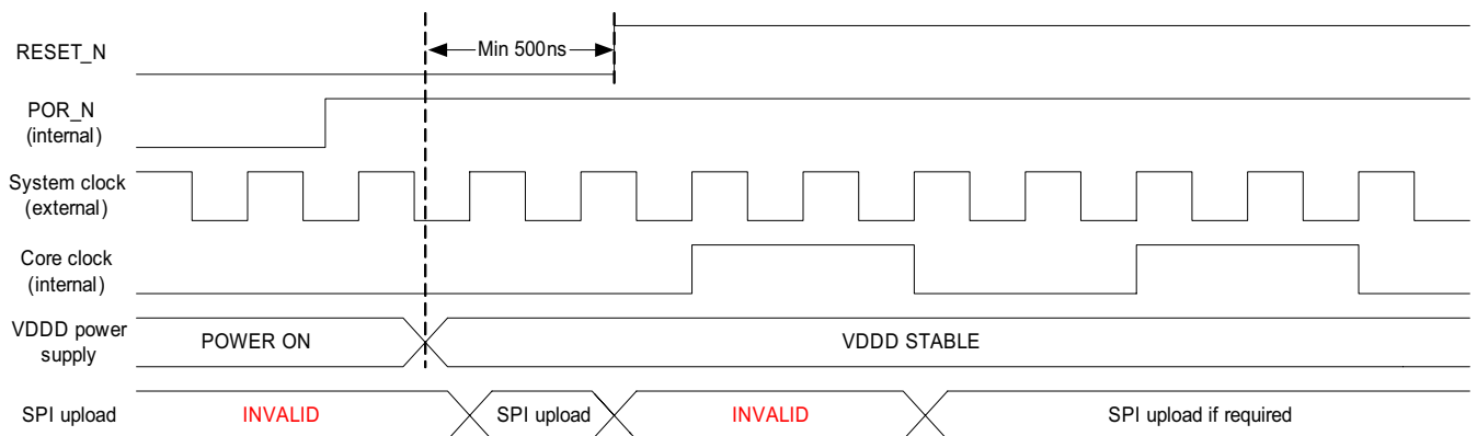
Figure 22. Start-Up Timing
