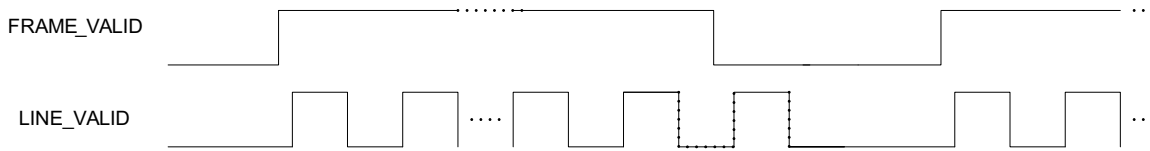
Figure 20. FRAME_VALID Timing
